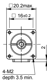
Front view and mounting
