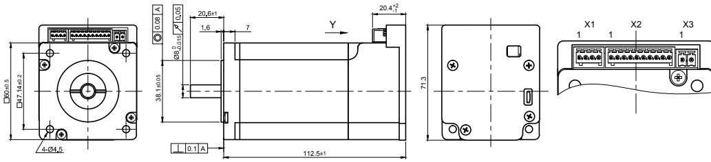
Front view and mounting
